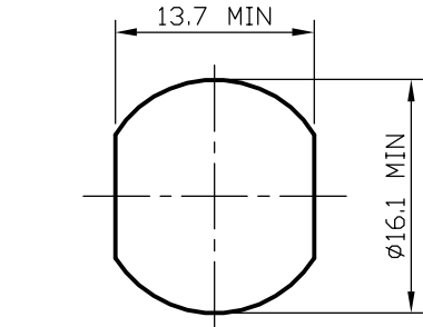
MOUNTING HOLES (REF)
