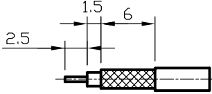
STRIP LENGTHS (REF)
