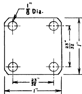
MOUNTING DIAGRAM
