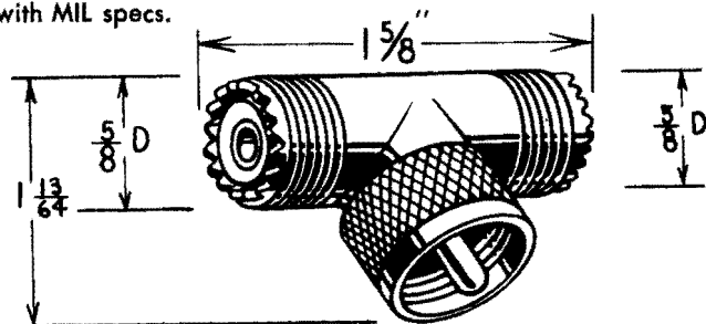
ADAPTER, TEE
