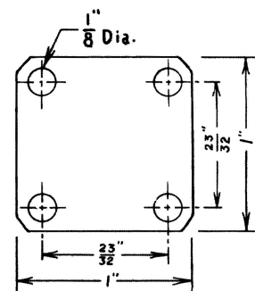
MOUNTING DIAGRAM
