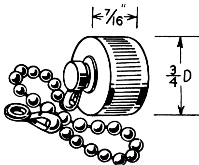
CAP & CHAIN
