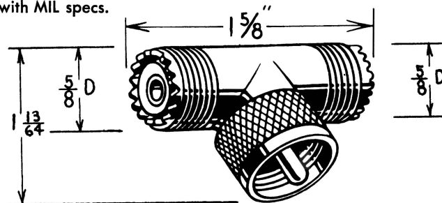
ADAPTER, TEE
