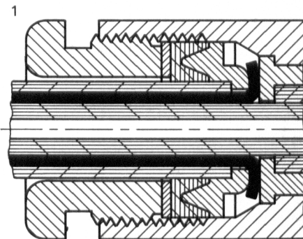
Cable-entry construction with sealed cable-entry unit
