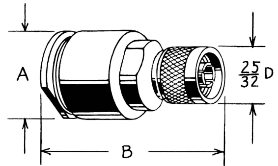
PLUGS — 50 ohm
