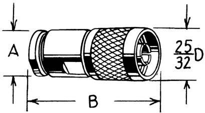
PLUGS — 50 ohm
