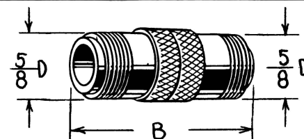
ADAPTERS — 50 ohm
