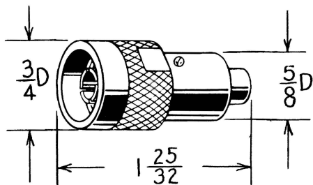
PLUG — 50 ohm
