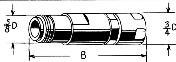
JACKS — 50 ohm
