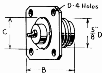
RECEPTACLES — 50 ohm
