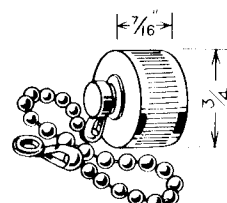
CAP & CHAIN
