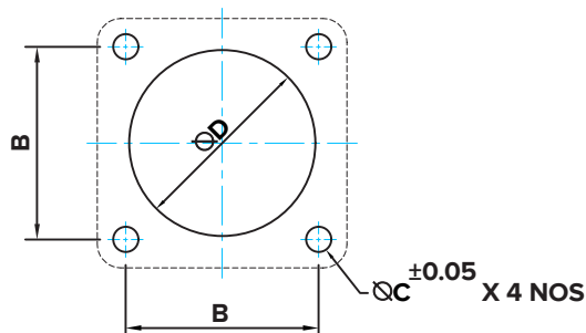
PANEL CUT OUT DIMENSIONS FOR SQUARE FLANGE RECEPTACLE (FRONT PANEL MOUNTING)
