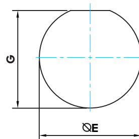
PANEL CUT OUT DIMENSIONS FOR JAM-NUT RECEPTACLE (REAR PANEL MOUNTING)
