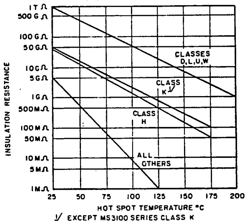
FIGURE 1. Minimum insulation resistance vs. hot spot temperature.
