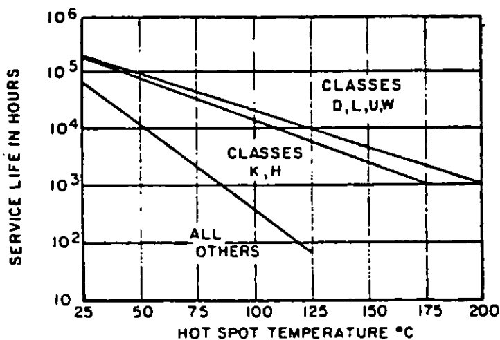
FIGURE 2. Service life vs. hot spot temperature.
