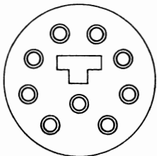
9 WAY LARGE
