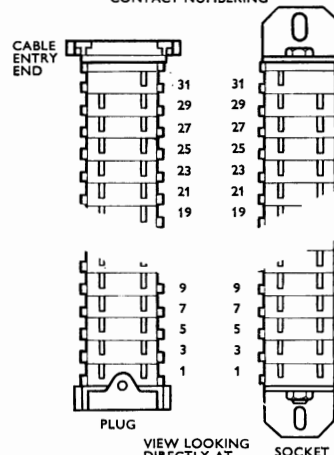
CONTACT NUMBERING
