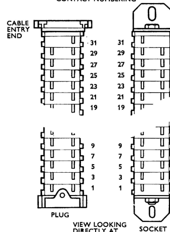
CONTACT NUMBERING
