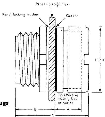
MAY BE MOUNTED FROM THE REAR OF THE PANEL ONLY
