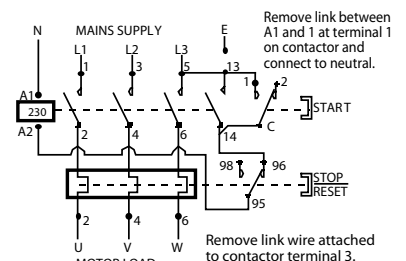
3 Phase 4 Wire Supply – 56MS230
