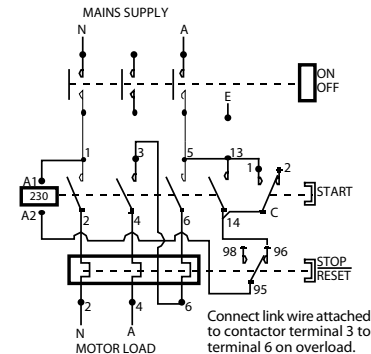
Single Phase & Neutral Supply – 56MS230SW
