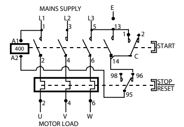
3 Phase 3 Wire Supply – 56MS400
