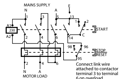
Single Phase & Neutral Supply – 56MS230
