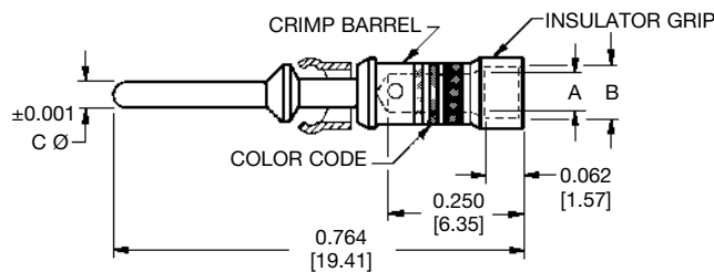
MALE CONTACT
