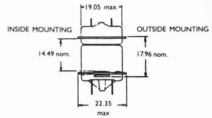
Barrier polarised plug and socket mated
