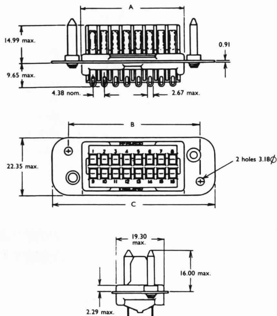
Plug
