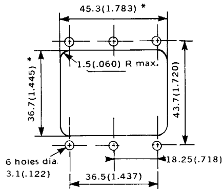
SHELL SIZE 1
