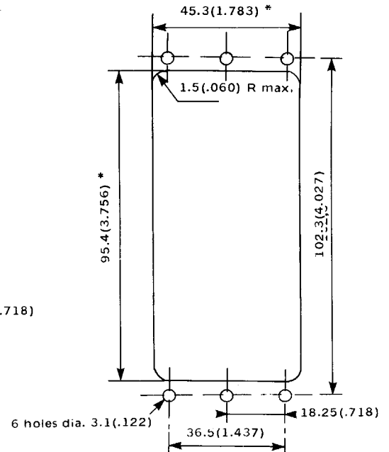
SHELL SIZE 3
