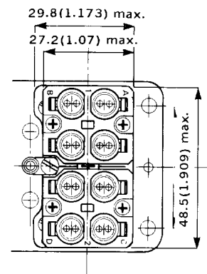
WIRING REAR FACE
