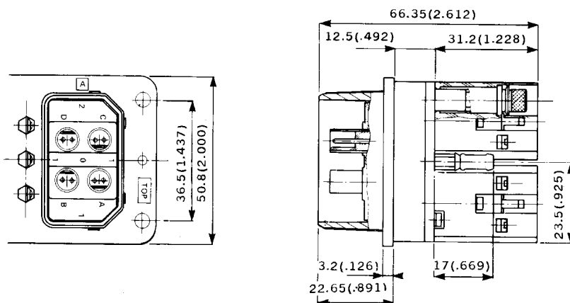
MATING FACE
