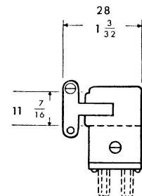
SIDE ENTRY
