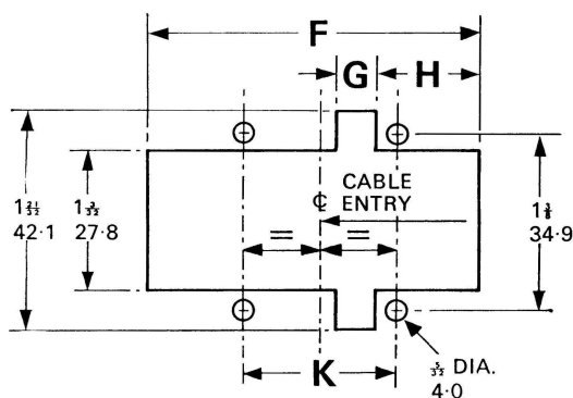
Type of Plug or Socket DIMENSIONS F G H K 18 POLES 2½ 51·6 ⅝ 7·5 ⅝ 13·9 1¼ 31·7 24 POLES 2½ 67·5 ⅝ 6·7 ⅝ 21·8 1¼ 31·7 33 POLES 3⅝ 91·3 ⅝ 6·7 ⅝ 21·8 2⅝ 55·6
