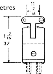
TOP ENTRY
