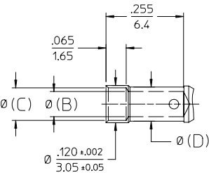
CRIMP
