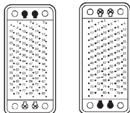
Plug Receptacle
