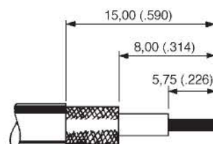
Part Number: 192945-4530
