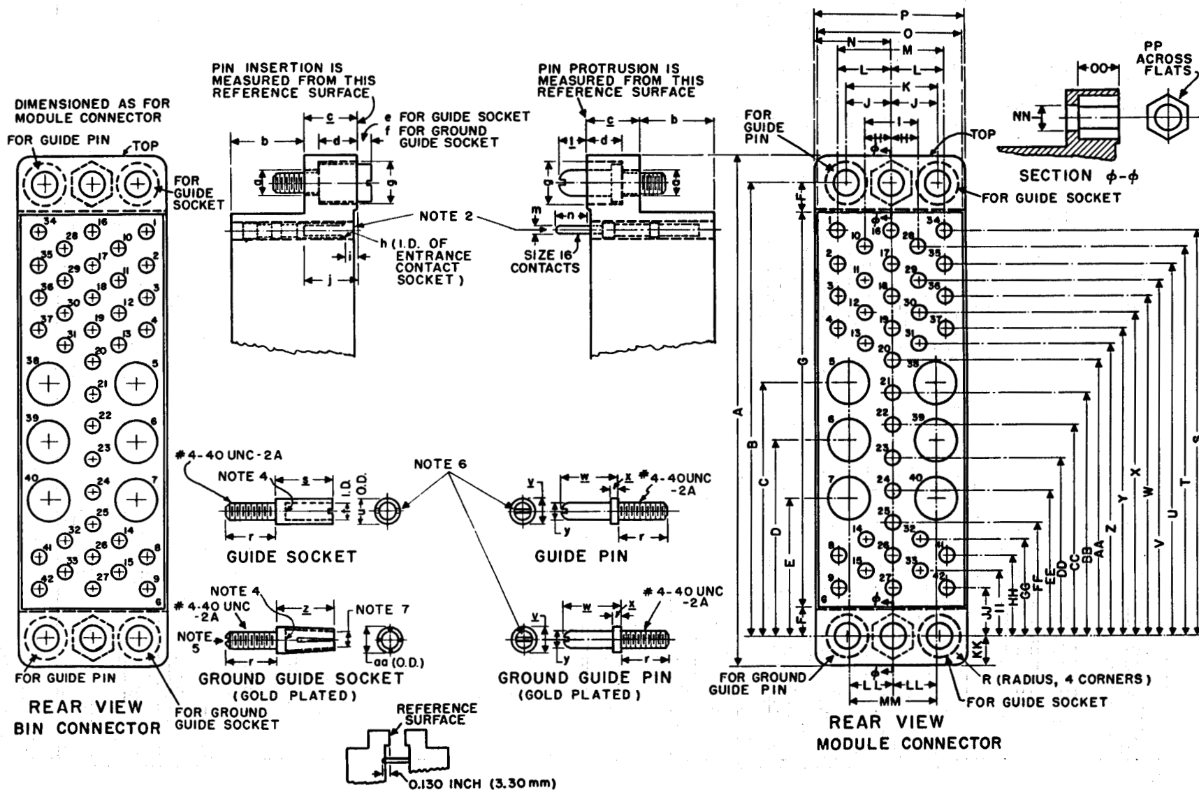
Figure 4a. Module and Bin Connector Details
