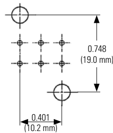
6 contacts
