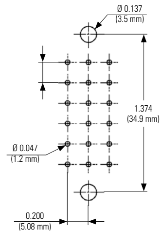
18 contacts
