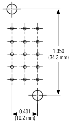
15 contacts
