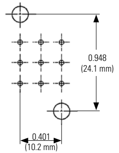
9 contacts
