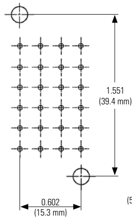
24 contacts
