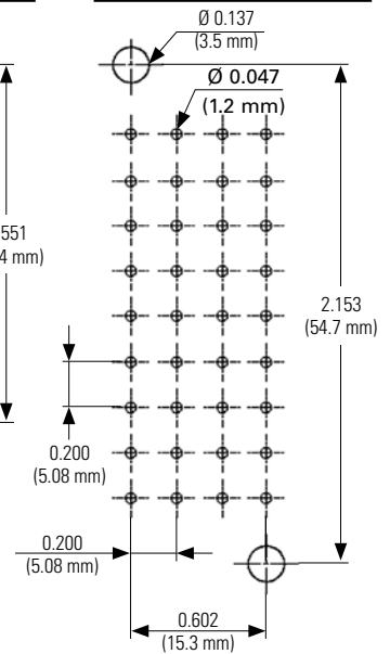
36 contacts
