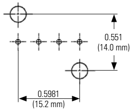
4 contacts
