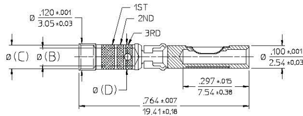
CATALOG NO'S M39029/35-275 & -276 SHOWN
