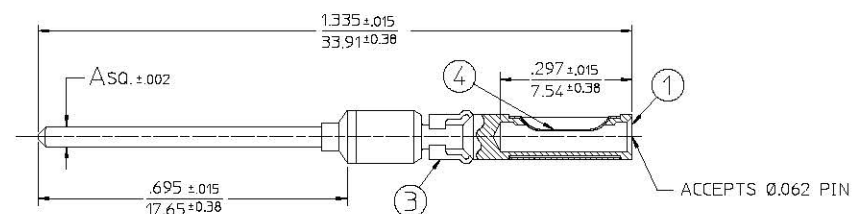
CATALOG NO'S 8105-Δ AND 8113-Δ SHOWN
