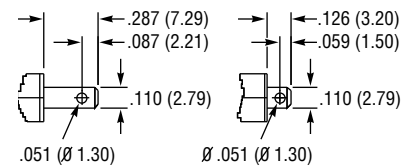
Auxiliary Switch Terminals
