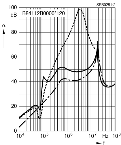
Filters for 20 A
