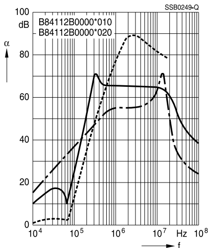
Filters for 6 A and 10 A
