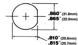
Mounting Hole B
