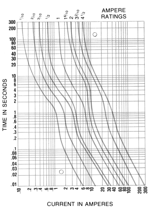
Fusetron MDA Dual-Element Fuses, 1/4" x 1 1/4" (6.4mm x 31.8mm)
