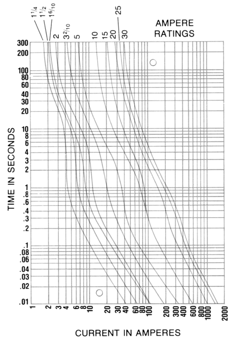
Fusetron MDL, MDV Dual-Element Fuses, 1/4" x 1 1/4" (6.4mm x 31.8mm)
