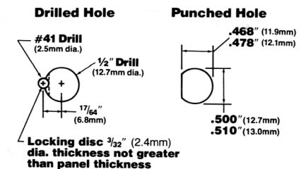
Mounting Hole A
