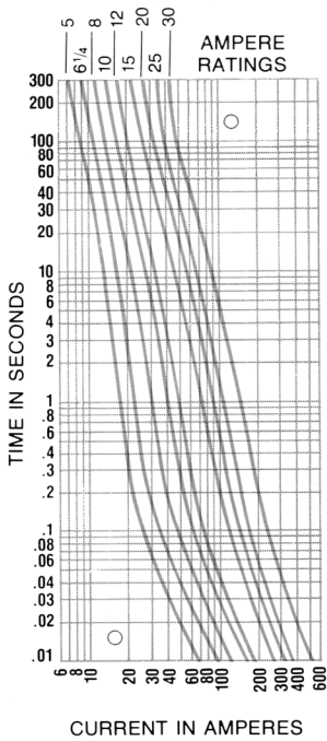
Type MDA Time-Delay Fuses, 1/4" x 1 1/4" (6.4mm x 31.8mm).
