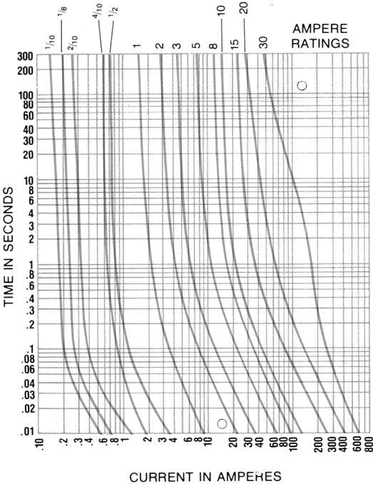
Limitron Fast-Acting KLM, KTK Fuses, 13/32" x 1 1/2" (10.3mm x 38.1mm)
