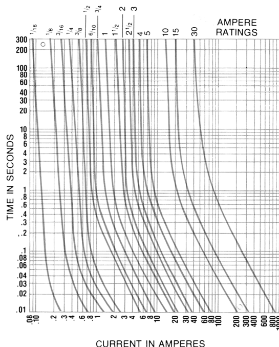
Type AGC Fuses, 1/4" x 1 1/4" (6.4mm x 31.8mm)
