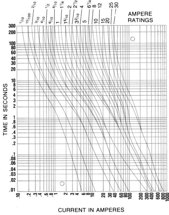
Fusetron FNM Dual-Element Fuses, 13/32" x 1 1/2" (10.3mm x 38.1mm)
