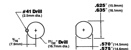
Mounting Hole D
