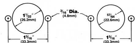
Mounting Hole C
