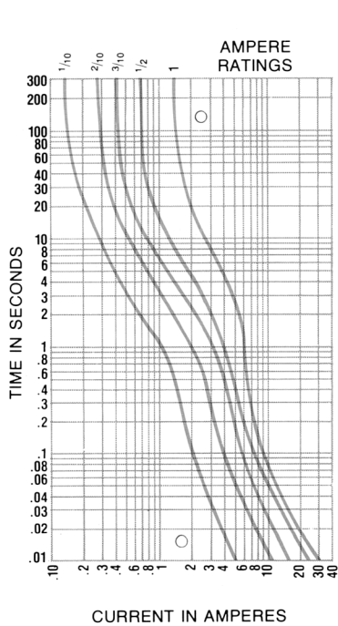
Fusetron MDL, MDV Dual-Element Fuses, 1/4" x 1 1/4" (6.4mm x 31.8mm)
