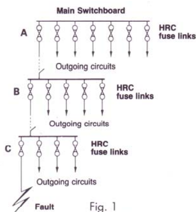
Fig. 1 Typical 3 phase (shown single line) distribution system
