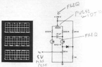
Fig. 2.28. Square Wave Generator.
