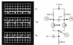
Fig. 3.25. Typical Monostable Multivibrator Operation.
