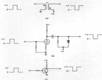
Fig. 3.13. "NOT" Circuits.
