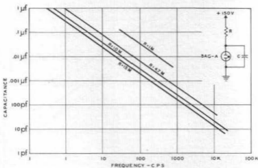
Fig. 2.8. Operating Frequencies as a Function of Resistance and Capacitance. (SAG-A at 150V)
