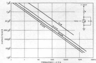
Fig. 2.7. Operating Frequencies as a Function of Resistance and Capacitance. (SAG-A at 100V)
