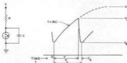
Fig. 2.2. Single Cycle of Typical Sawtooth Output
