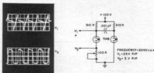
Fig. 2.25. Glow Lamp Multivibrator.
