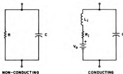
Fig. 1.4. Equivalent Circuits for the Glow Lamp
