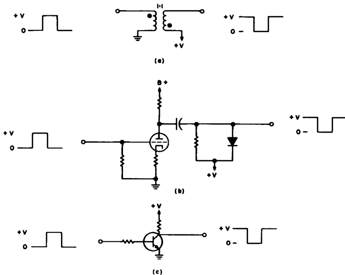
Fig. 3.13. "NOT" Circuits.
