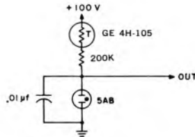
Fig. 2.33. Temperature Indicator.
