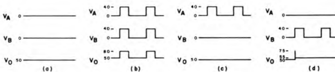
Fig. 3.6. "AND" Gate Waveforms.
