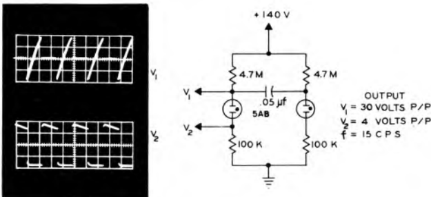
Fig. 2.21. Modified Multivibrator and Outputs.
