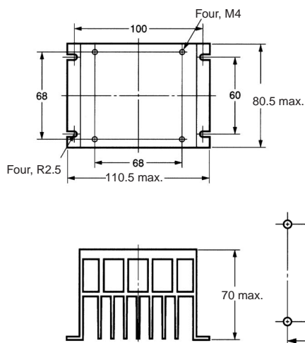
Mounting Holes
