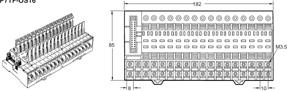
For Output (NPN, + Common) P7TF-OS16
