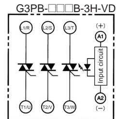
Terminal Arrangement/ Internal Circuit Diagram
