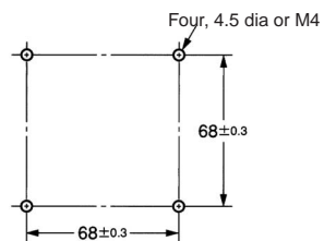
Mounting Holes
