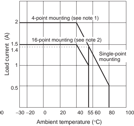
G3R-ODX02SN-UTU (4 to 60 VDC)
