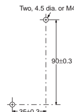
Mounting Holes
