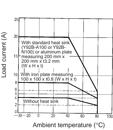
G3NA-220B/420B
