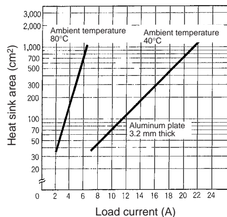
G3NA-220B
