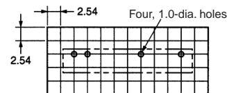
Terminal Arrangement (Bottom View)
