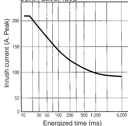
G3NA-220B/420B
