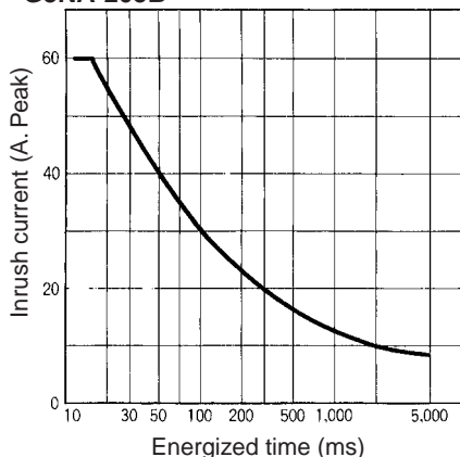
G3NA-205B
