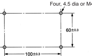
Mounting Holes
