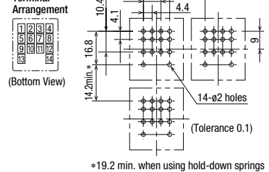
Terminal Arrangement (Bottom View)
