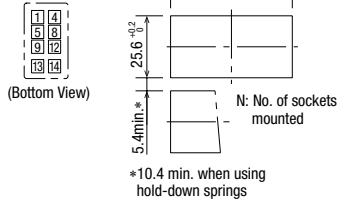
Terminal Arrangement (Bottom View)
