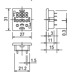
Terminal Arrangement (Bottom View)
