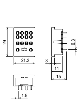
Terminal Arrangement (Bottom View)
