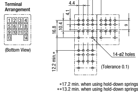
Terminal Arrangement (Bottom View)
