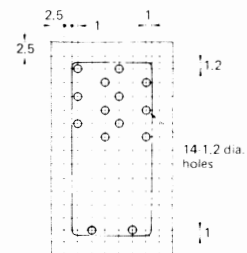
P3A-14P (Bottom view)
