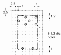
P3A-08P (Bottom view)
