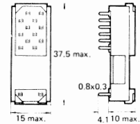
P3A-14P (Bottom view)
