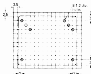
Mounting holes
