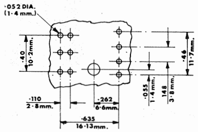
SPECIAL GRID FOR DIRECT MOUNTING TOP VIEW
