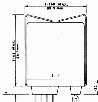
SOCKET TERMINALS WITH .04 X .08 (1mm X 2mm.) ELONGATED HOLES.
