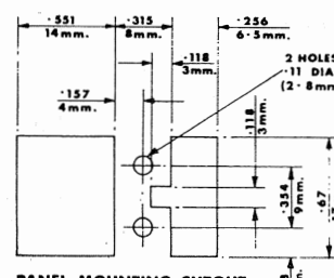
PANEL MOUNTING CUTOUT
