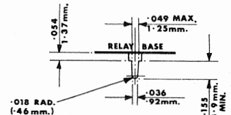
DIRECT MOUNTED PRINTED CIRCUIT TERMINAL
