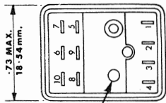
PIP .09 DIA. (2.3mm.) X .025/.02 (.63mm. X .5mm.) HIGH.
