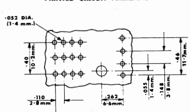
SPECIAL GRID FOR DIRECT MOUNTING TOP VIEW
