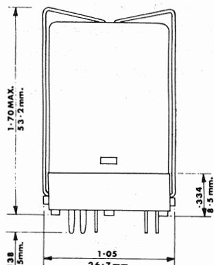
RELAY & PRINTED CIRCUIT SOCKET
