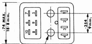
2 HOLES .12 DIA. (3mm.) STANDARD SOCKET UNDERNEATH VIEW
