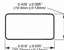
PANEL CUT-OUT FOR SOCKET
