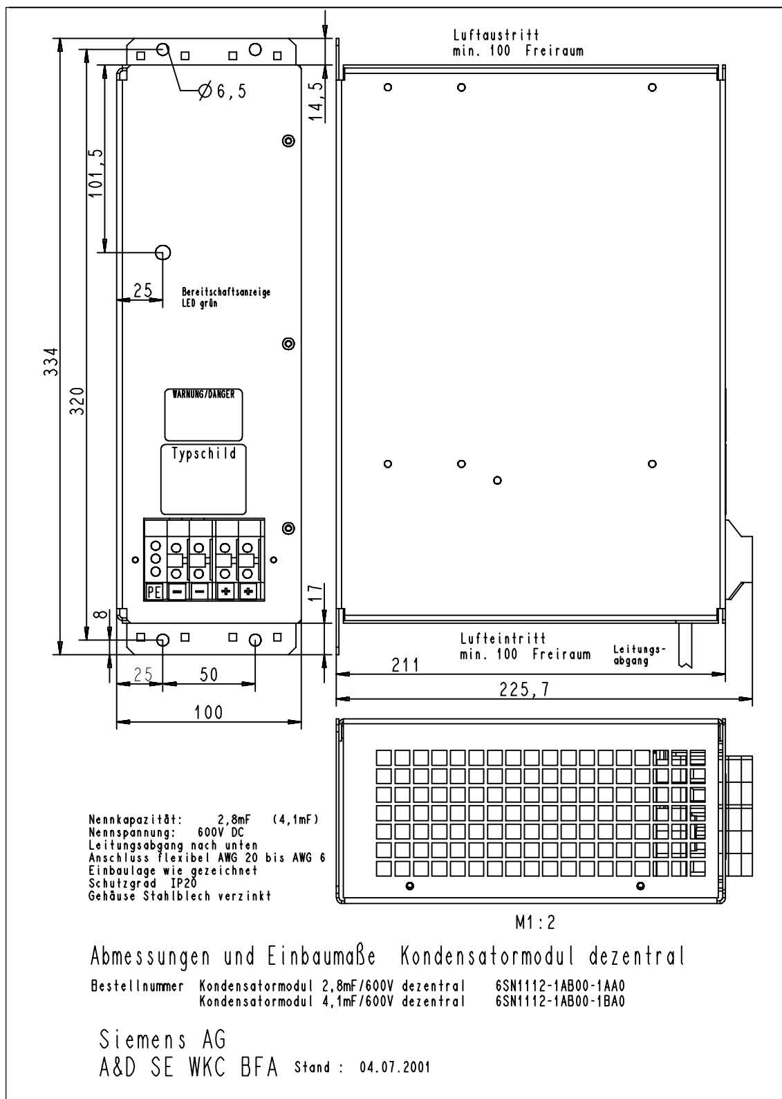
Fig. 12-55 Distributed capacitor modules, 6SN1112-1AB00-1xA0
