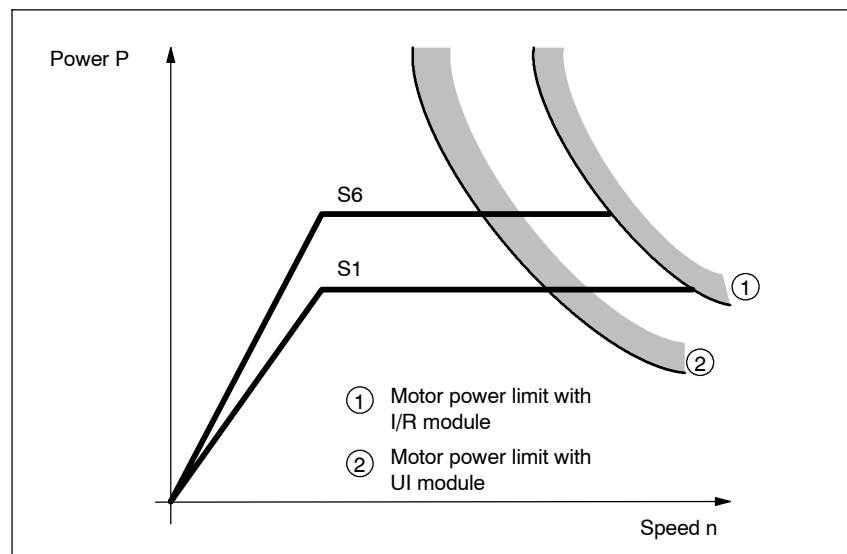
Fig. 4-10 Speed/power graph
