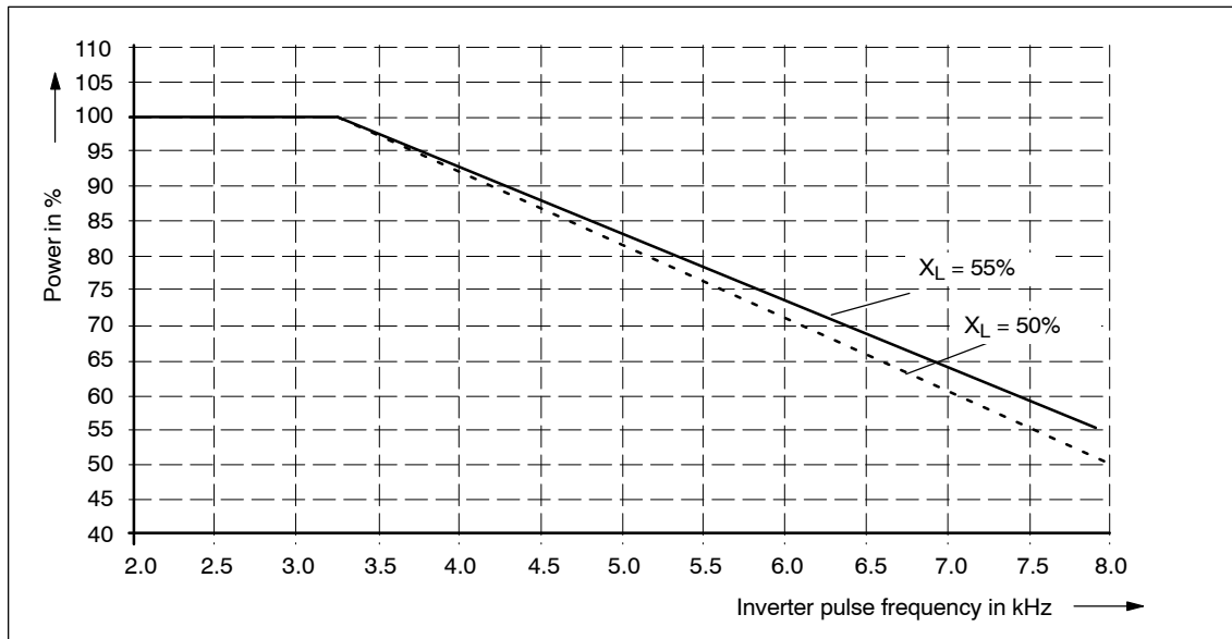
Fig. 4-6 Power as a function of the inverter pulse frequency for MSD–IM and MSD–SRM
