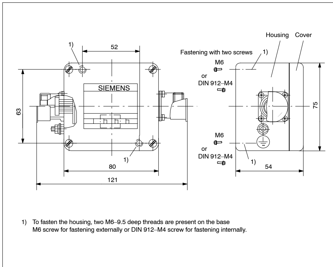
Fig. 12-51 Signal amplifier electronics SVE, 6SN1115-0AA12-0AA0
