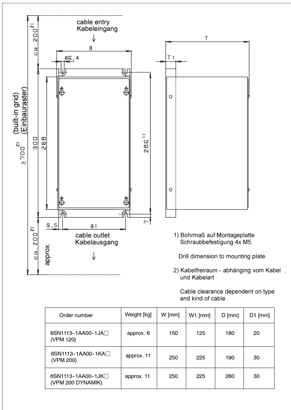
Fig. 12-61 VPM 120/VPM 200/VPM 200 DYNAMIK, dimension drawing
