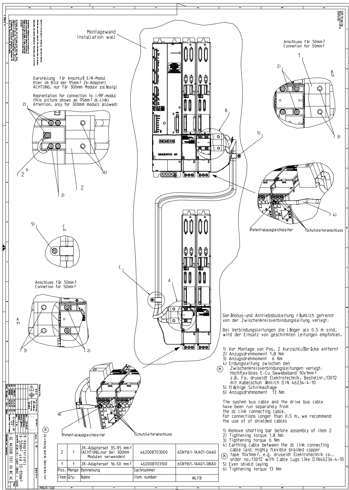
Fig. 12-56 DC link adapter set 16...50 mm² and 35...95 mm² 6SN1161-1AA01-0BA0/-0AA0
