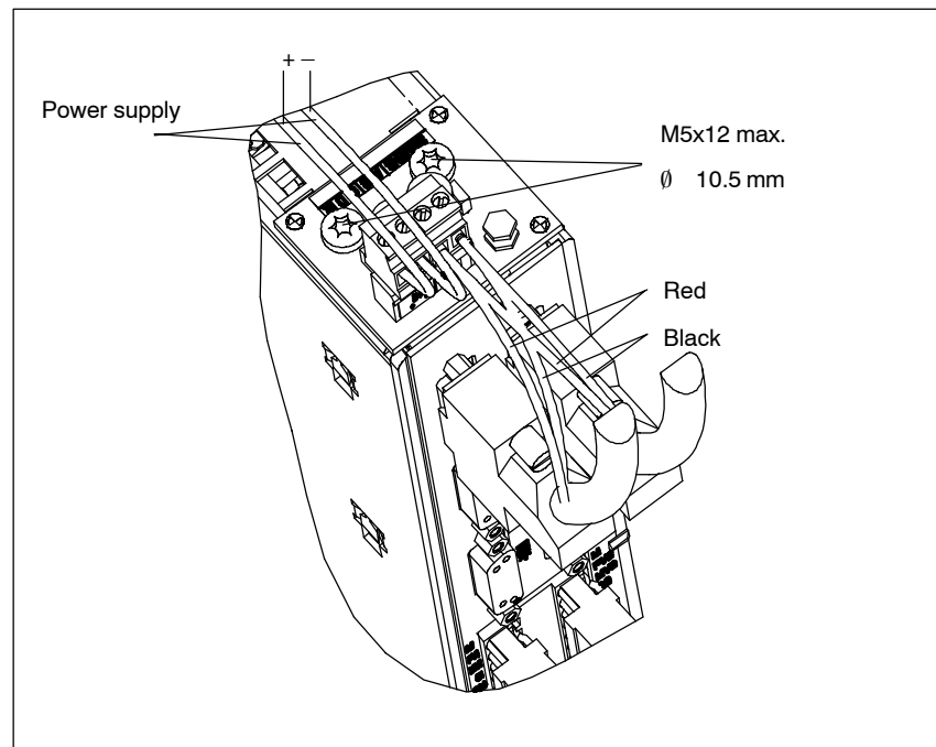
Fig. 3-9 Connection example for the "HLA module" control board
