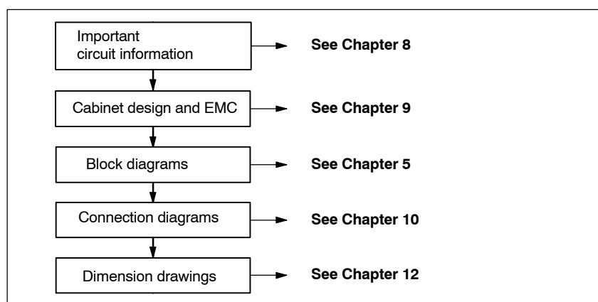
Fig. 1-5 Connecting-up
