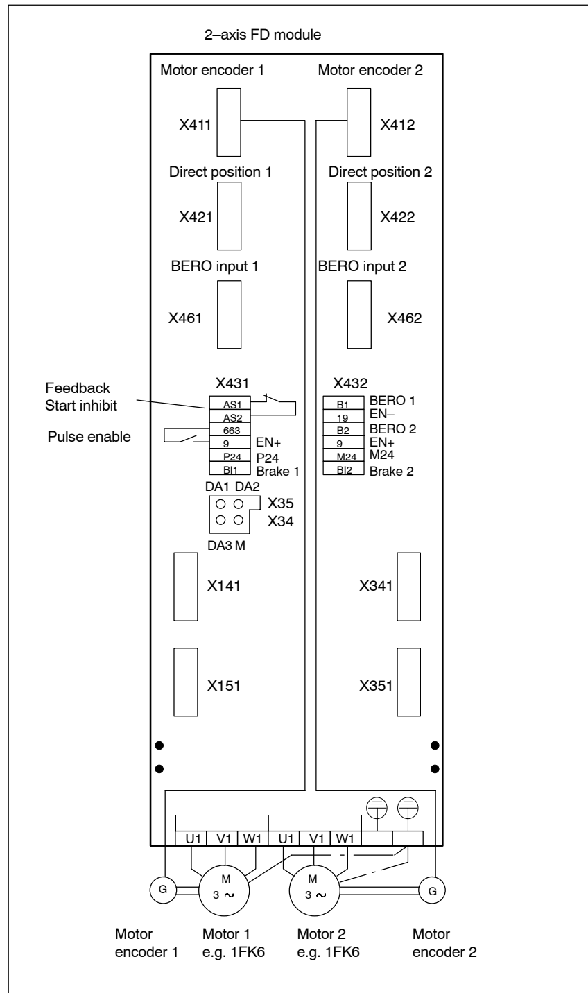
Fig. 8-9 Diagram showing the terminals of the VSA module with High Performance/High Standard
