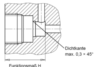
Figure 2: Location hole threaded-body type
