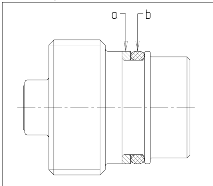
Figure 3: Position of the seal kit.
