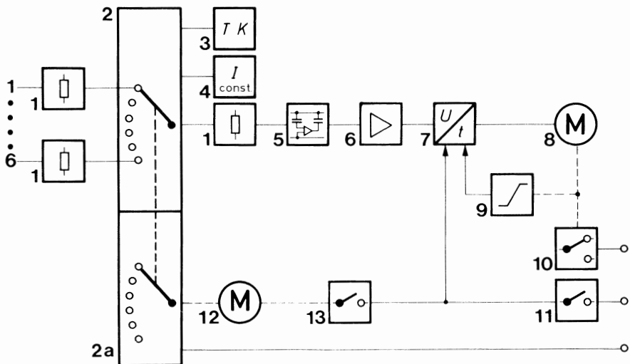
Fig. 1 Block diagram of Motorized Point Recorder 144
