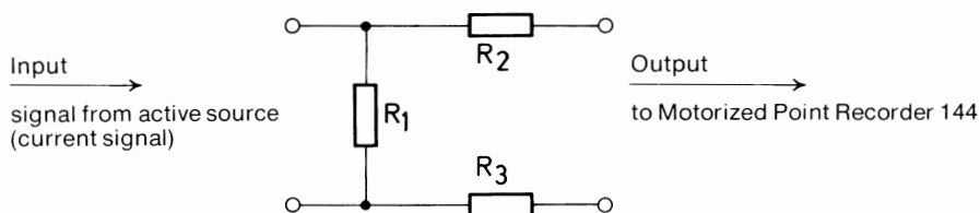
Fig. 12 Circuit of matching module for voltage and current limiting
