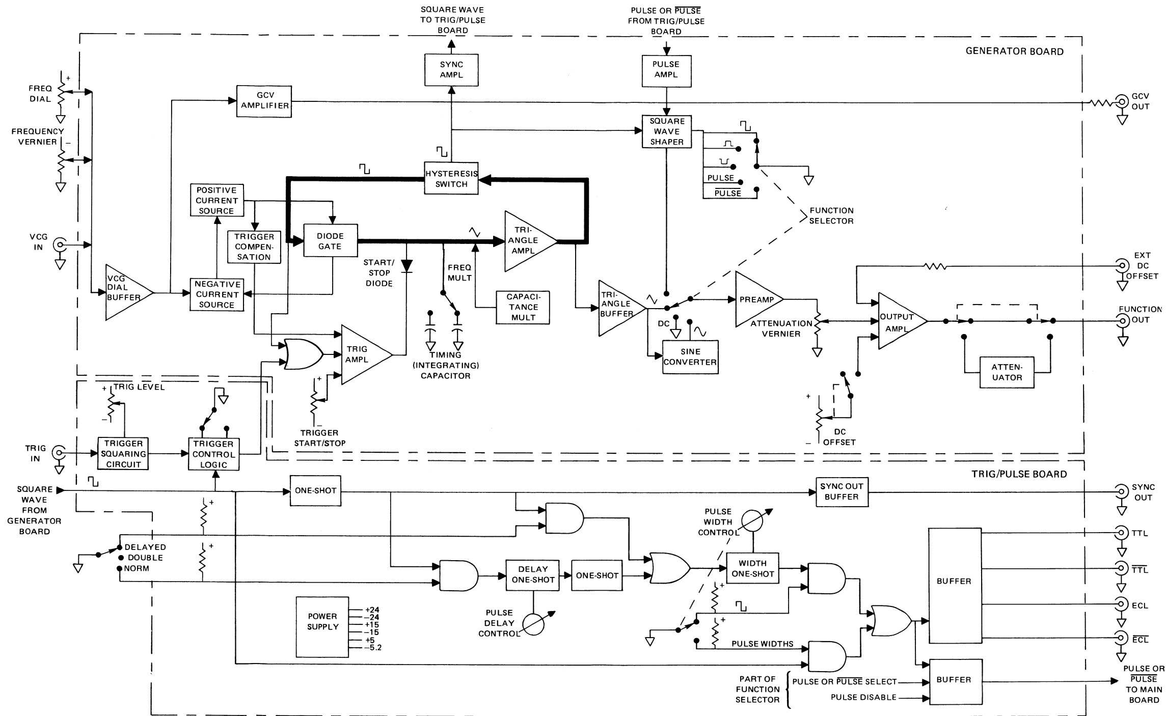
Figure 4-1. Overall Block Diagram
