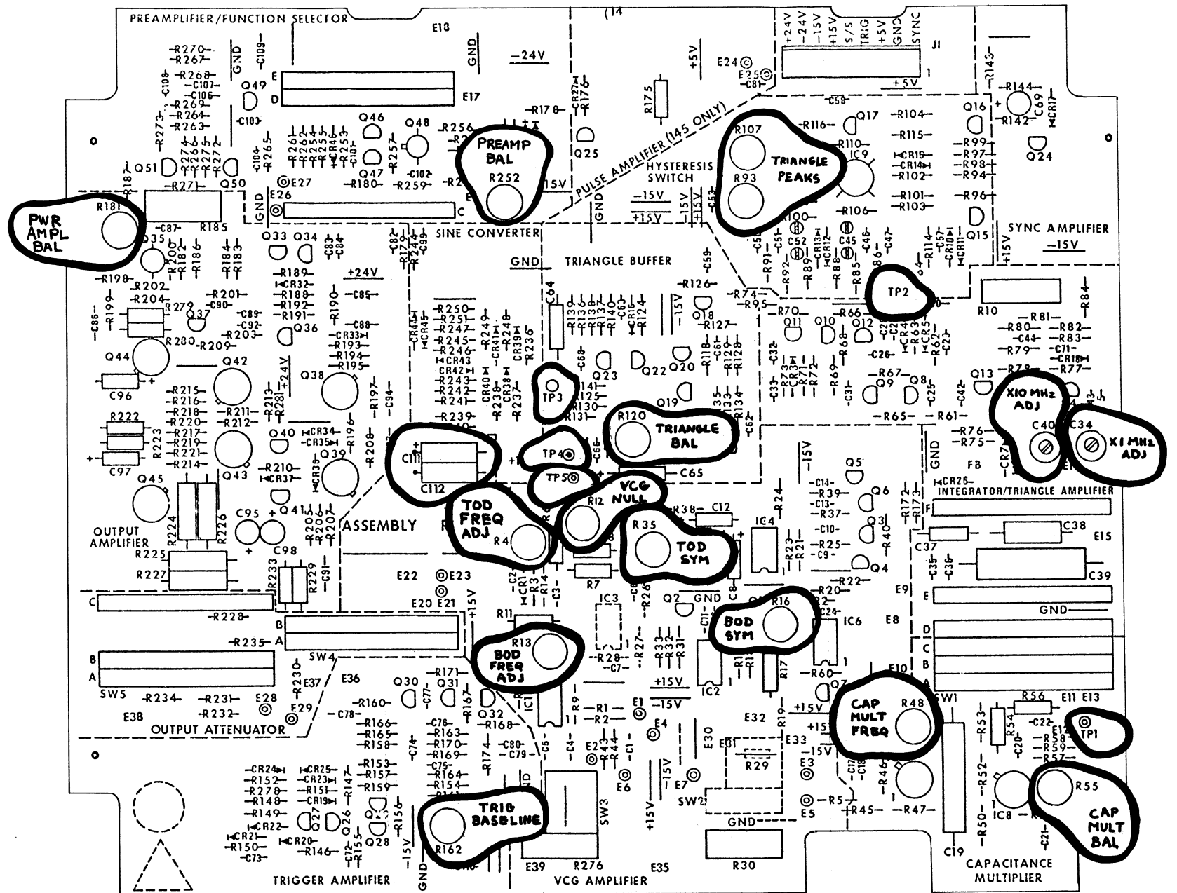
Figure 5-1. Generator Board
