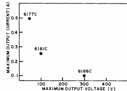
Precision Current Sources (page 251)
