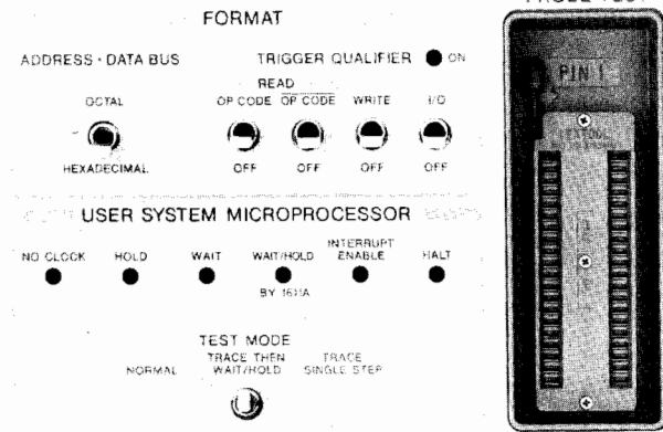
Opt A80 8080 \mu P Personality Module
