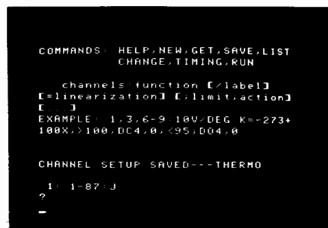
Level 2: Line entry . . . no computer language required . . . just enter data logger information
