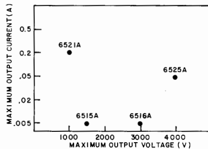
High Voltage Power Supplies (page 252)
