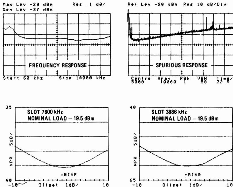
Figure 1. Back-to-back performance characteristics of wideband modulator and demodulator.
