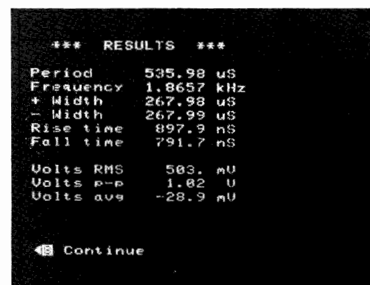
An example of the results obtained when using the Automatic Waveform Measurement Program (bottom photo).
