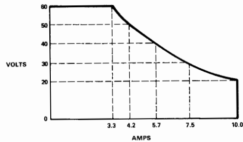
Autoranging operating area for the 6024A
