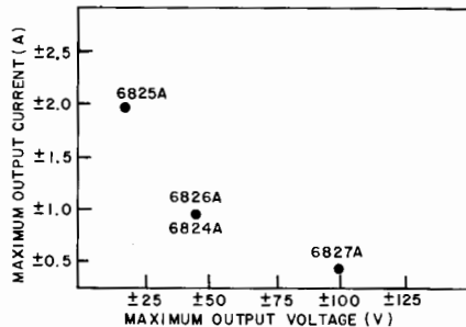
Bipolar Power Supply/Amplifiers (page 249)
