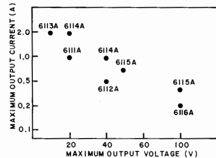
Precision Voltage Sources (page 250)
