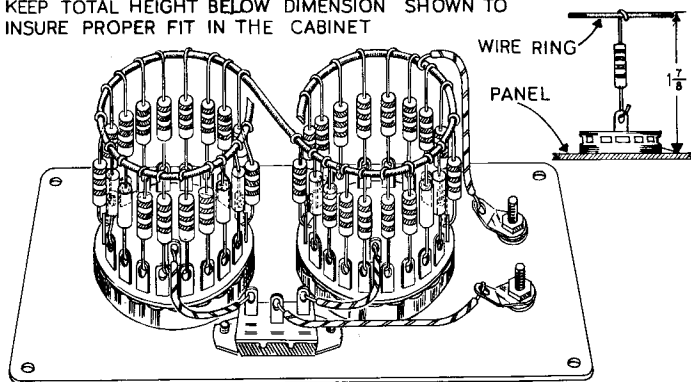
WIRING PICTORIAL
