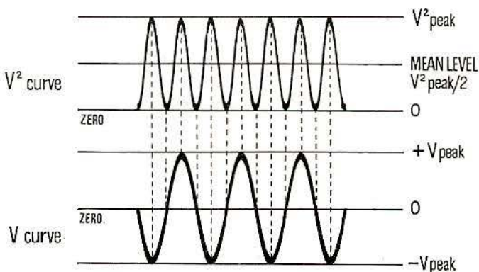
Fig. 5 Sinewave voltage and power waveforms.
