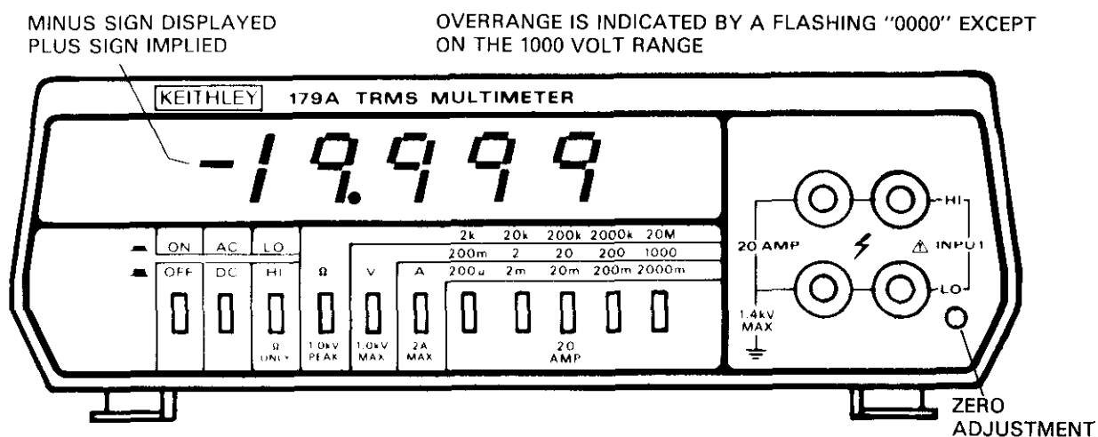
Figure 2-2. Model 179A Front Panel View
