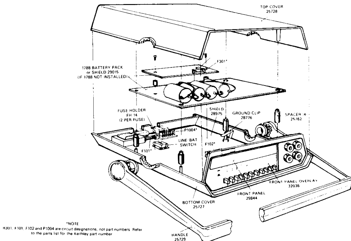
Figure 6-1. Miscellaneous Parts
