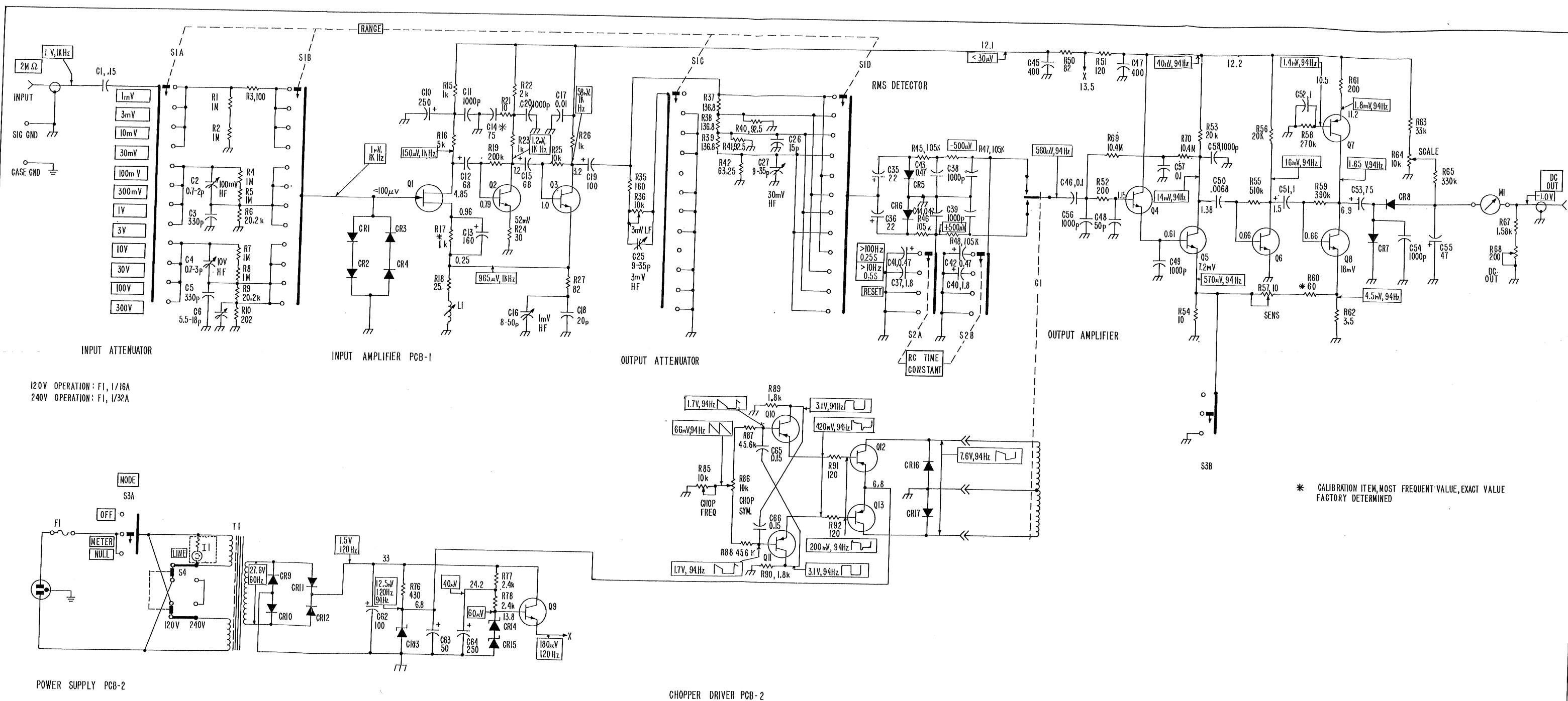
Fig. 22. Wiring Diagram of Model 323-01 True RMS Voltmeters Drawing No. ME-3450L
