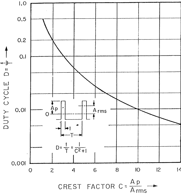
Fig. 5. Crest Factor vs. Duty Cycle for Pulse Trains
