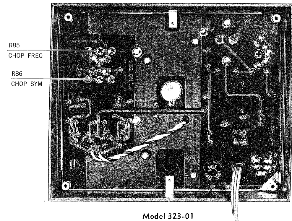
Fig. 14. Instrument Adjustments, Rear View
