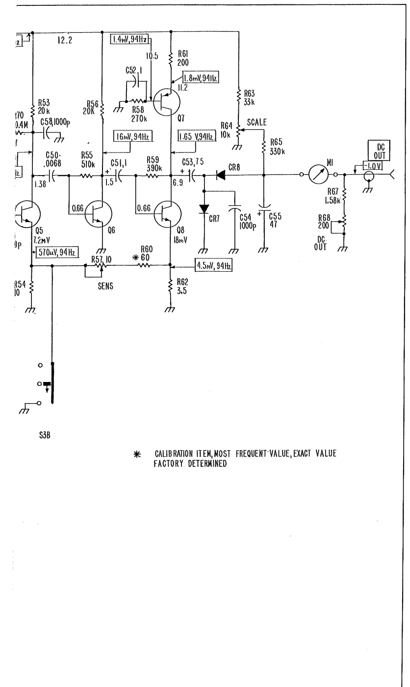
Fig. 22. Wiring Diagram of Model 323-01 True RMS Voltmeters Drawing No. ME-3450L
