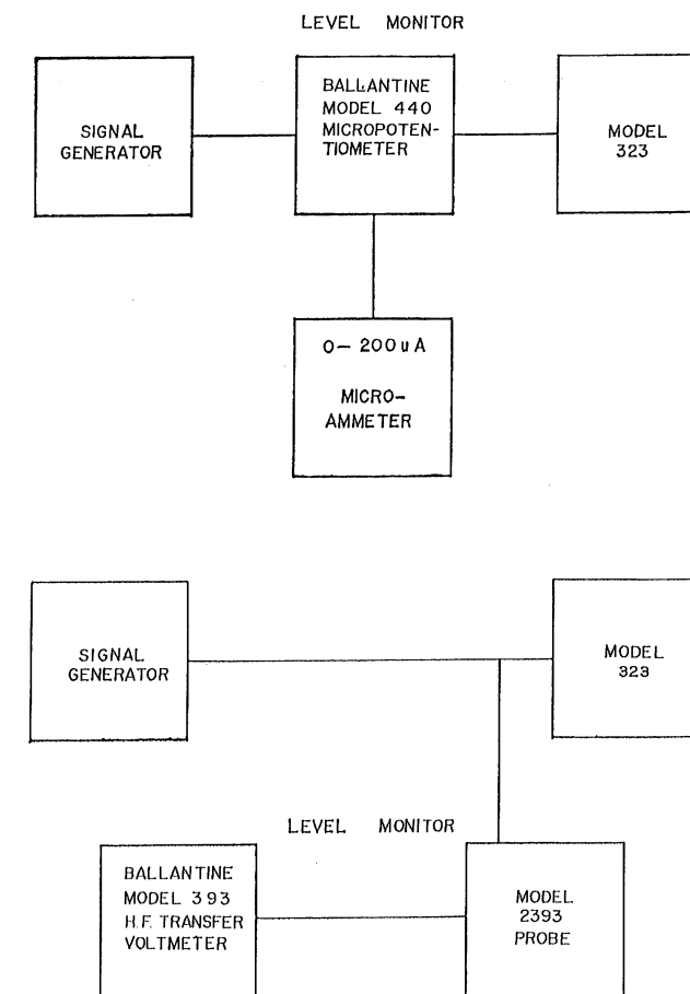
Fig. 16. Frequency Response Check
