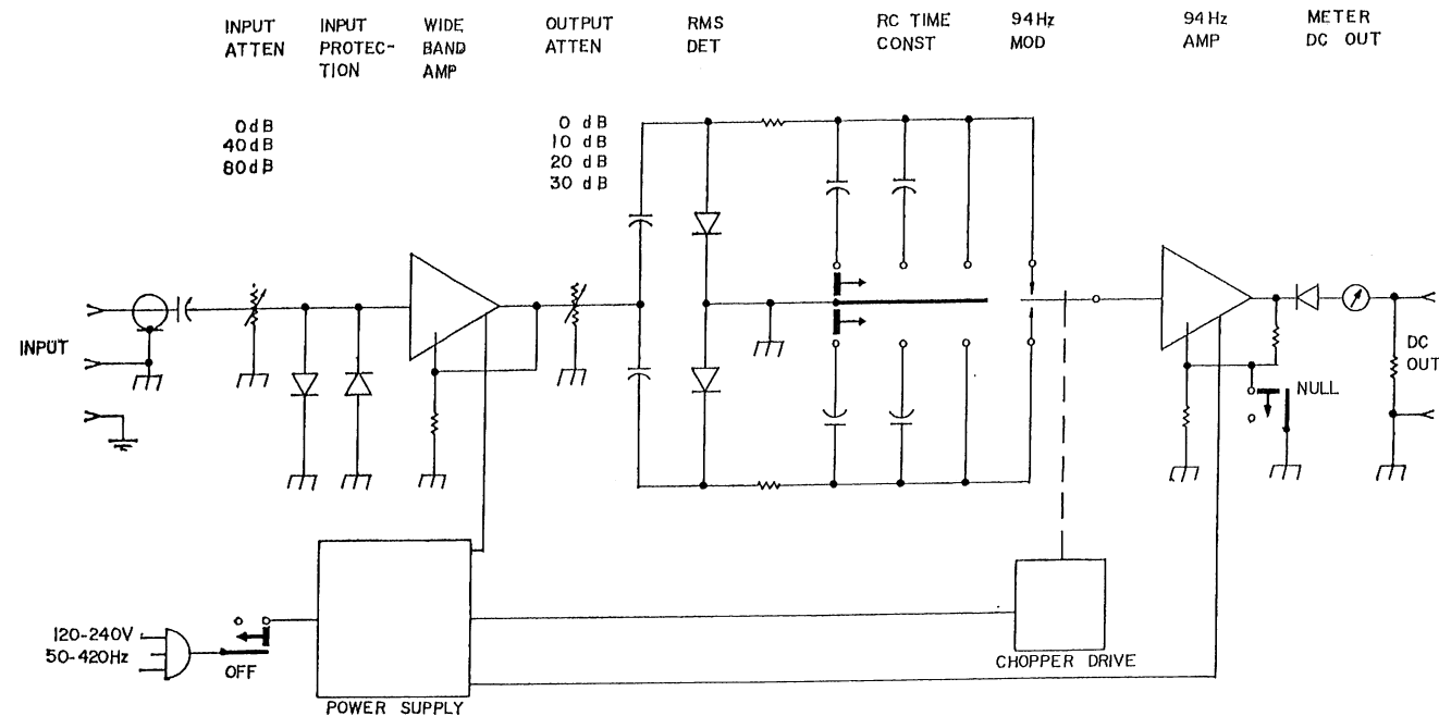
Fig. 11. Simplified Schematic, Models 323, 323-01
