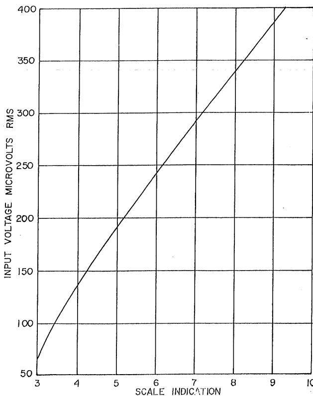
Fig. 9. Typical Calibration of 1 mV Range in NULL Mode
