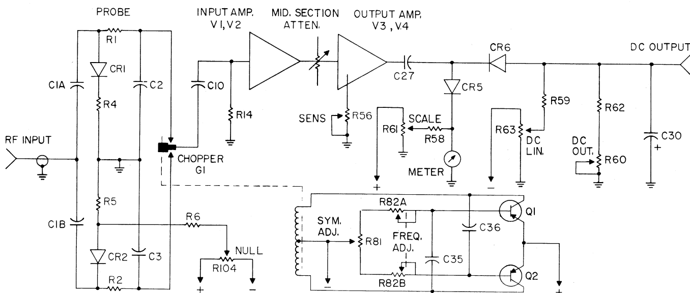
Fig. 7. Model 340 Simplified Schematic
