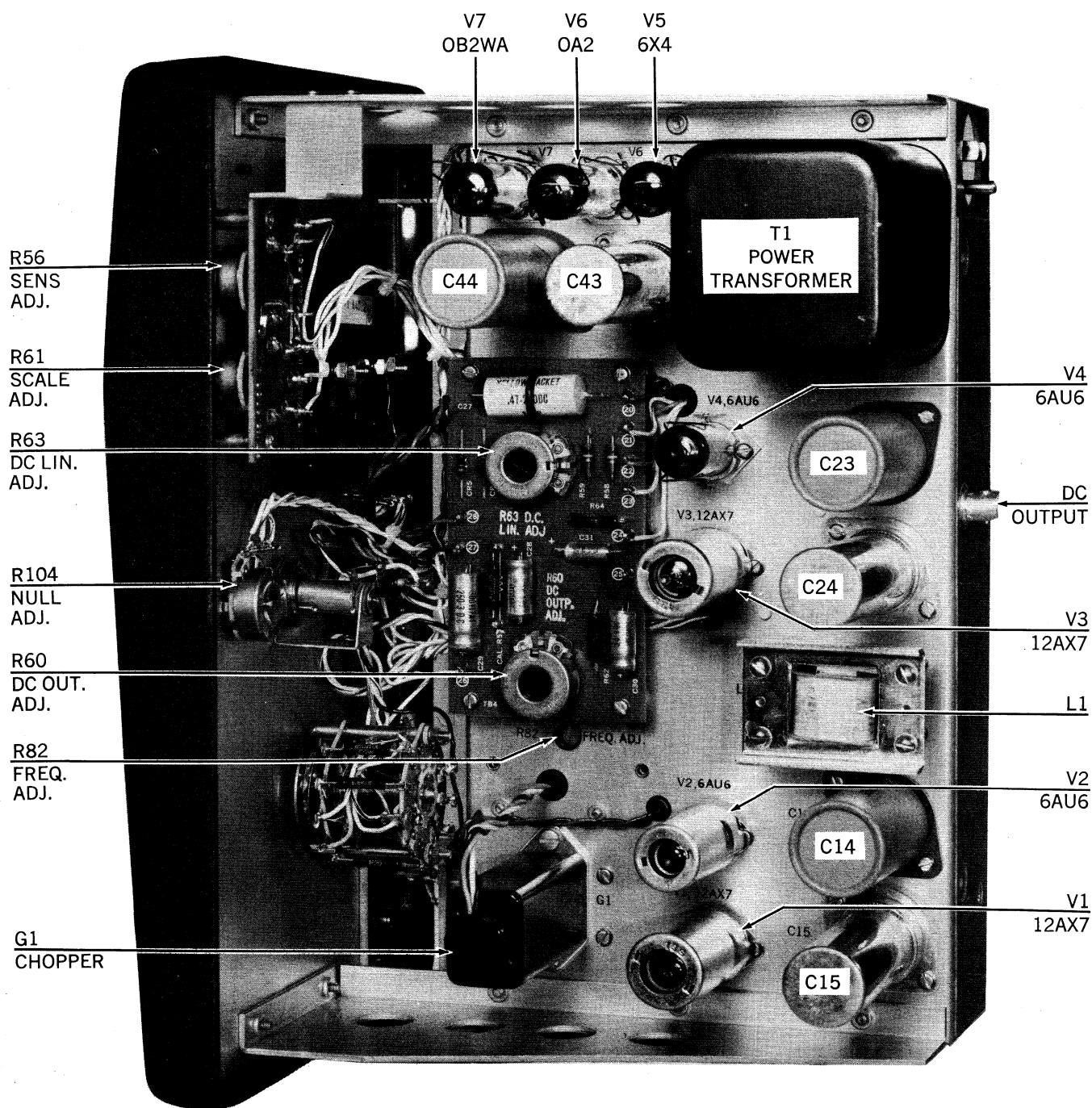
Fig. 8. Model 340 — Right Hand Side View
