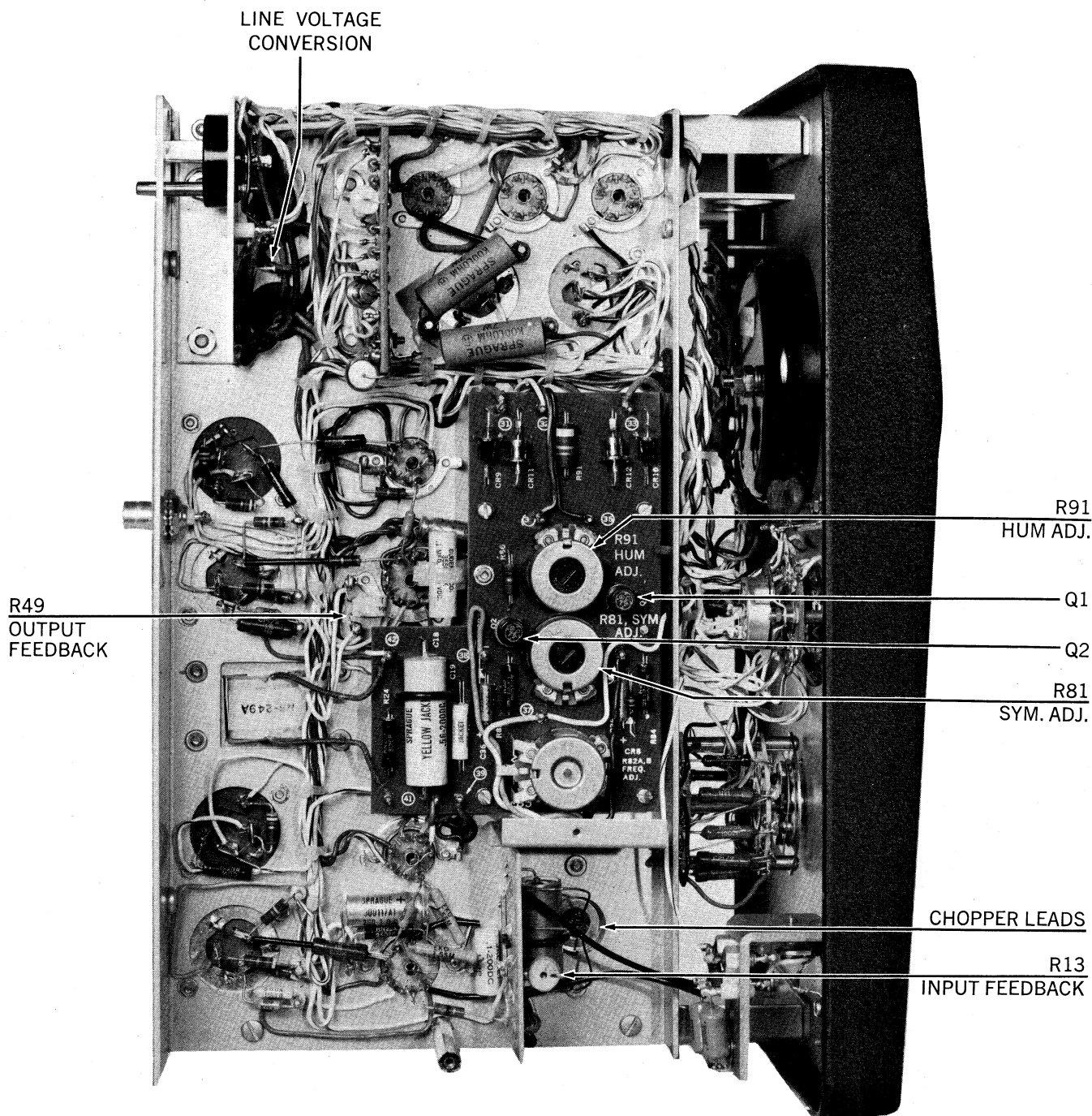
Figure 9. Model 340 — Left Hand Side View Input Shield Removed
