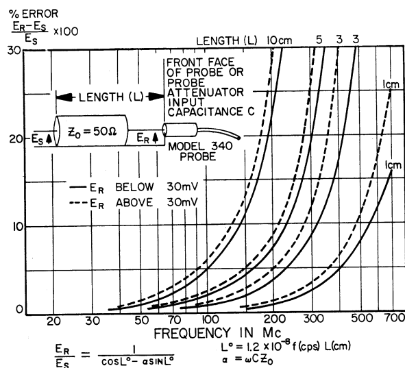
Fig. 5. Model 340 Transmission Line Errors
