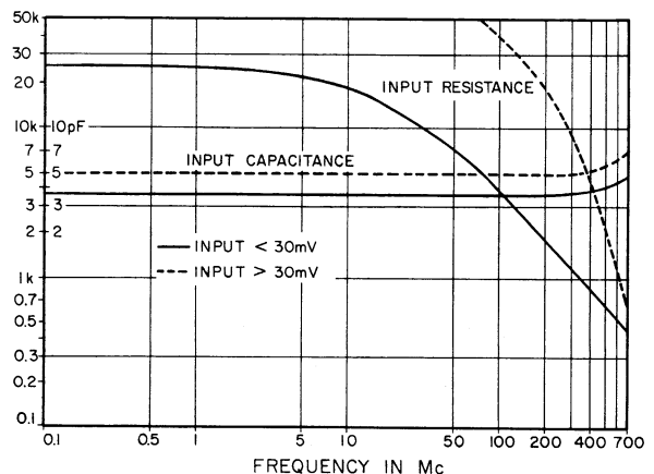
Fig. 4. Model 340 Input Impedance
