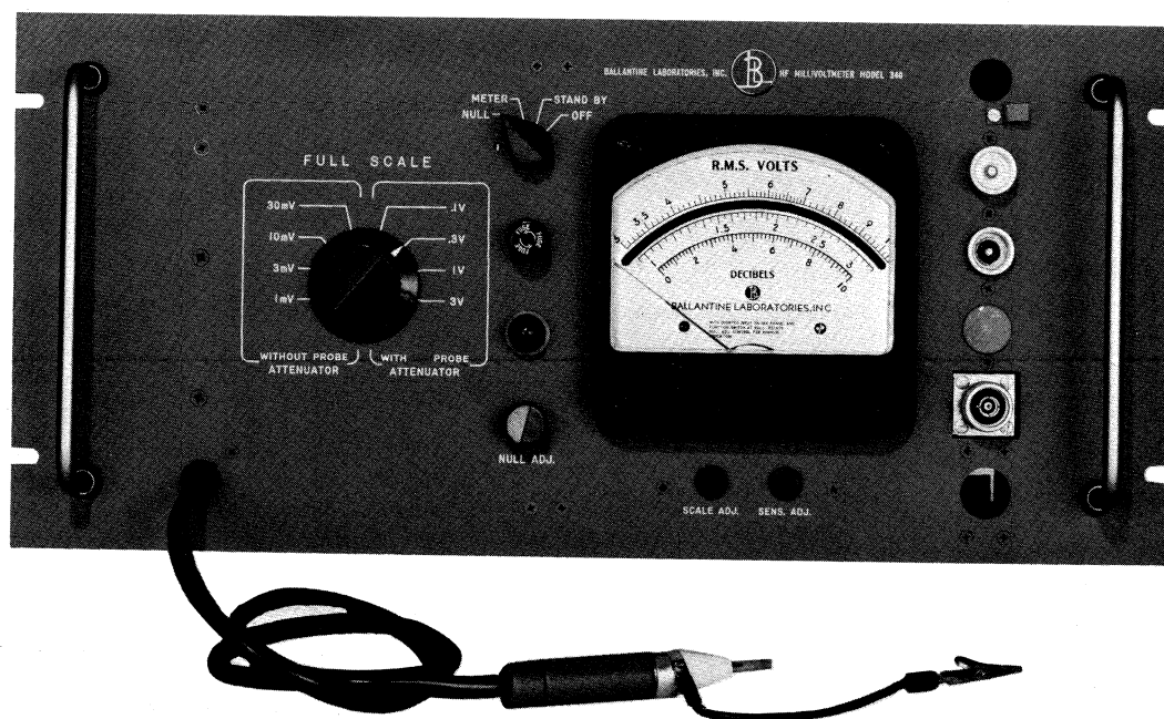
Figure 2. Rack Panel Mounted Ballantine Model 340-S/2 RF Millivoltmeter
