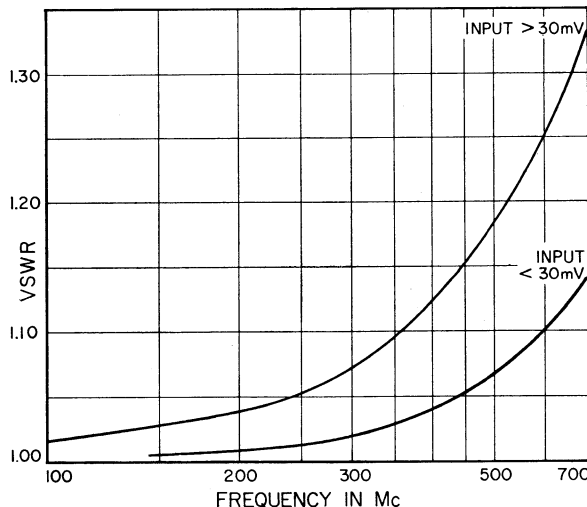
Fig. 6. Model 5340 VSWR
