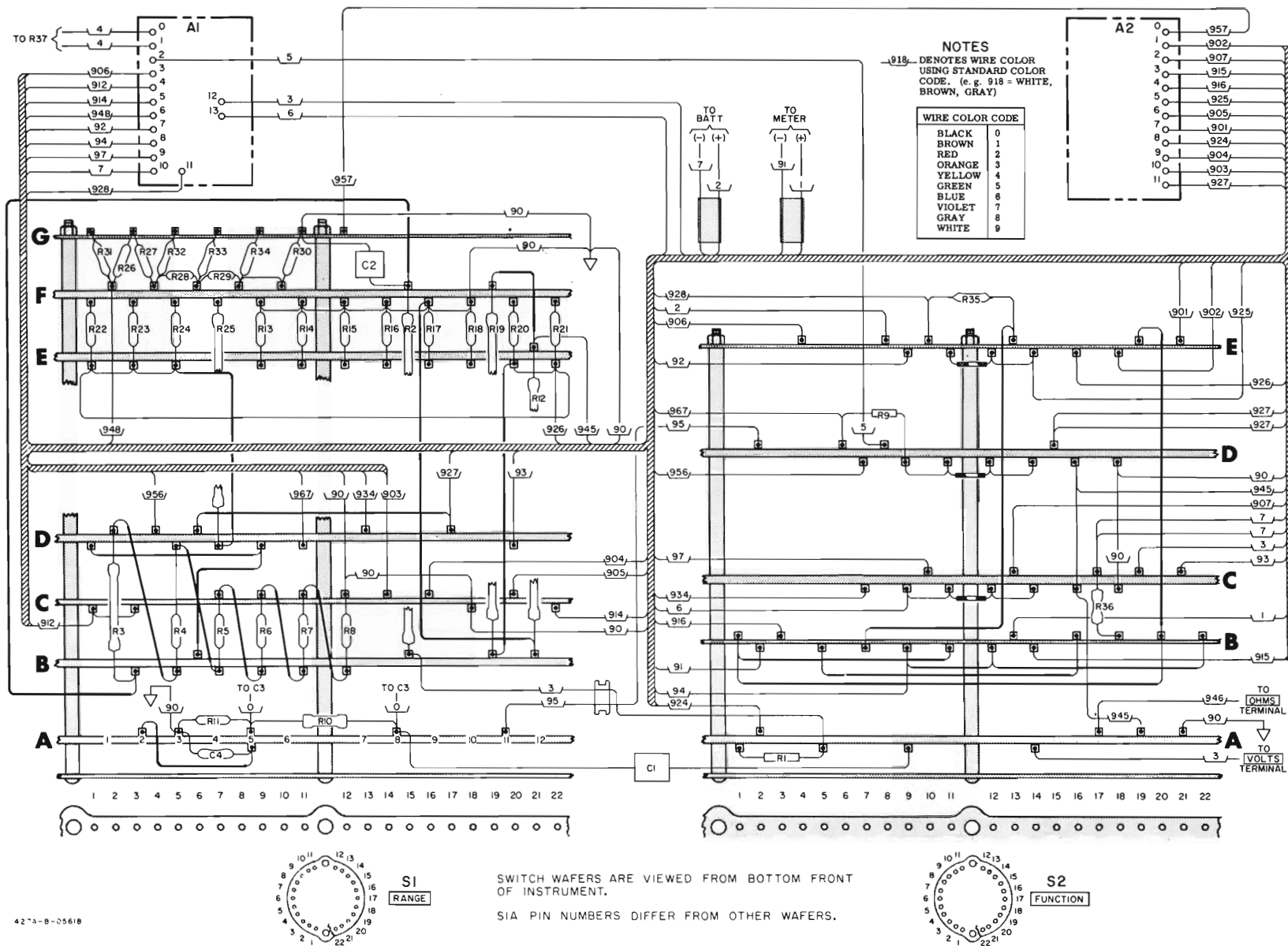
Figure 6-1. Location of Switch Components
