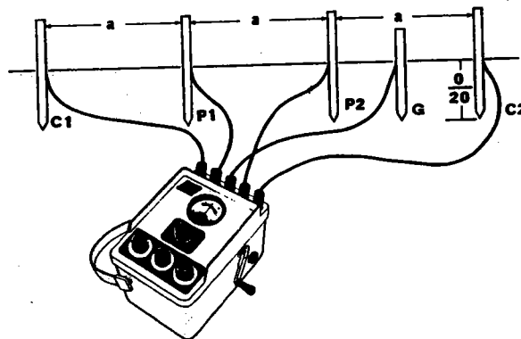
Figure 3-7. Connections for Measuring Earth Resistivity (Guard Terminal is used with Hand-Cranked Earth Tester Only).
