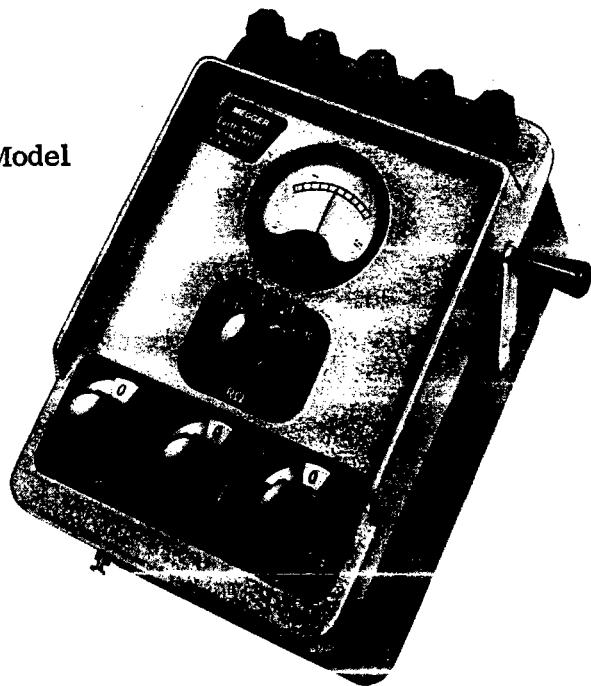
Figure 2-1. Megger Null Balance Earth Testers.
