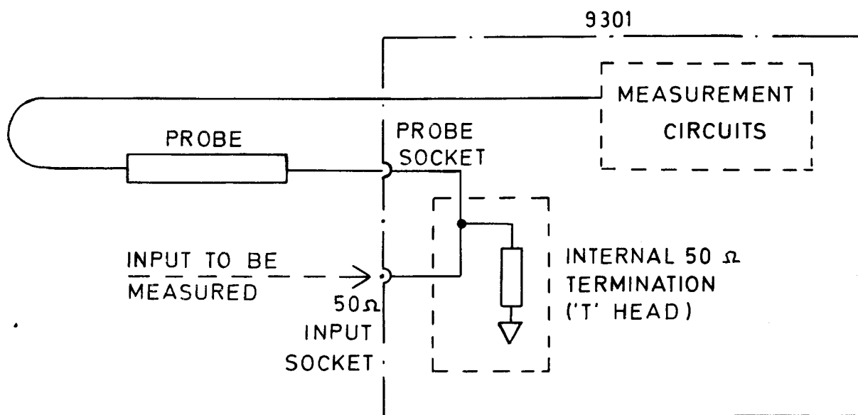
Probe And Input Connections For Internal 50 \Omega Termination
