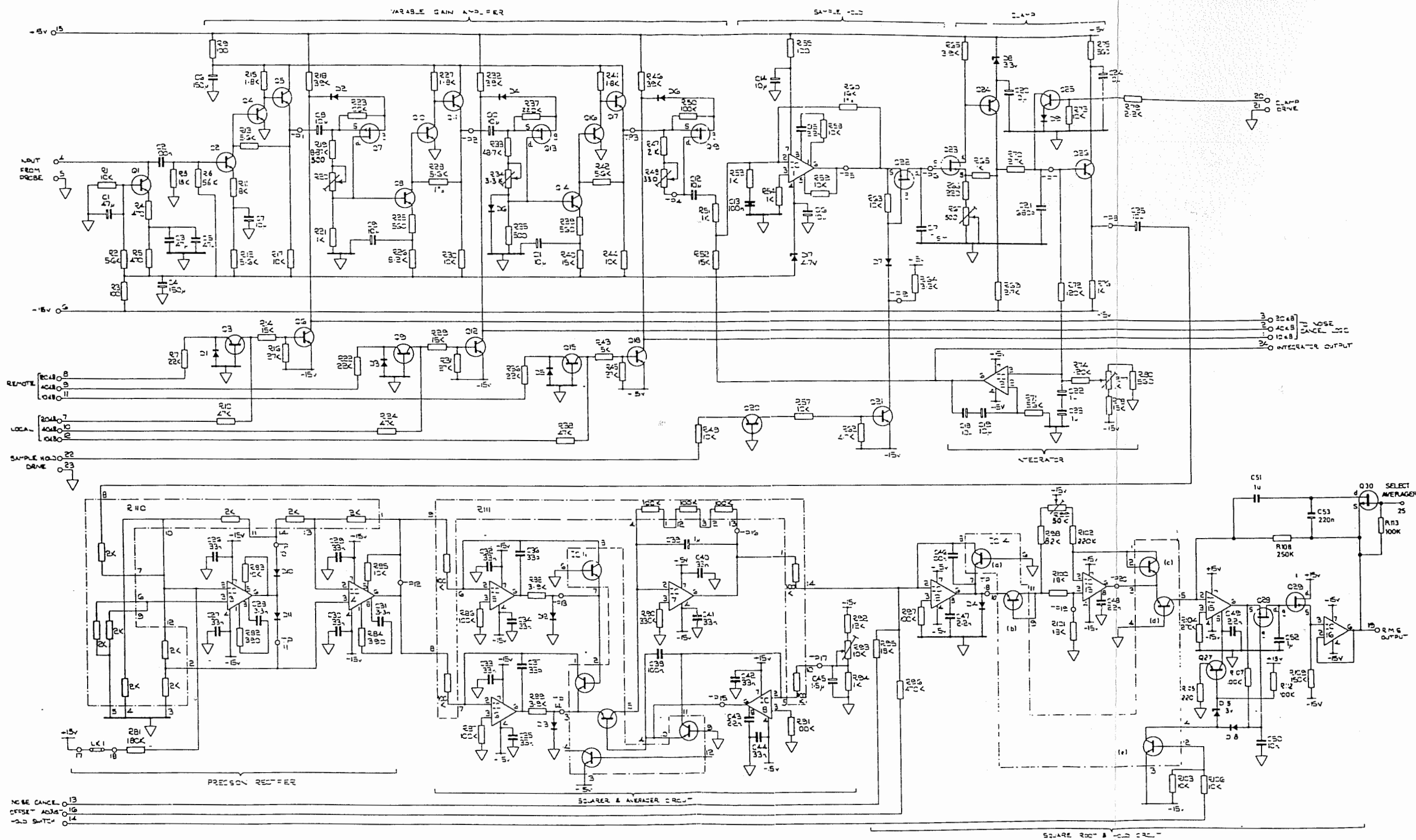
Circuit: Processor Assembly 19-0822
