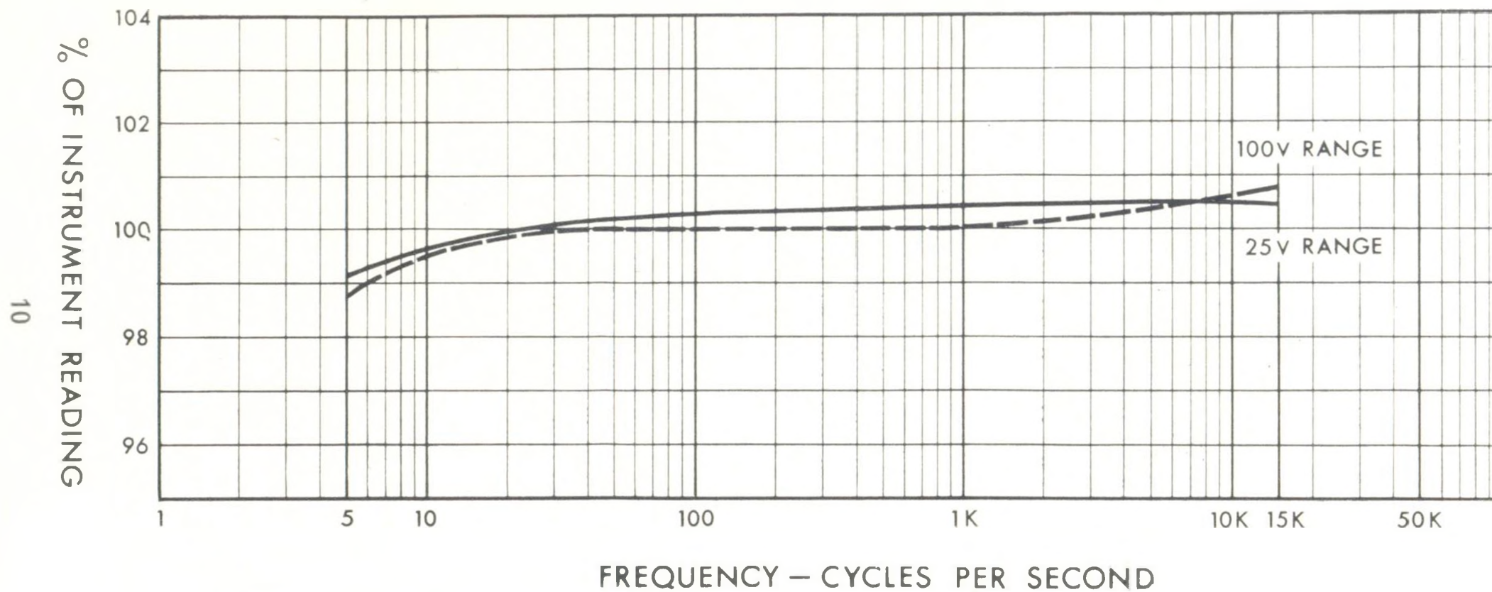
Fig. 1. Typical frequency response of Avometer Model 8 Mk III on 25 and 100V ranges
